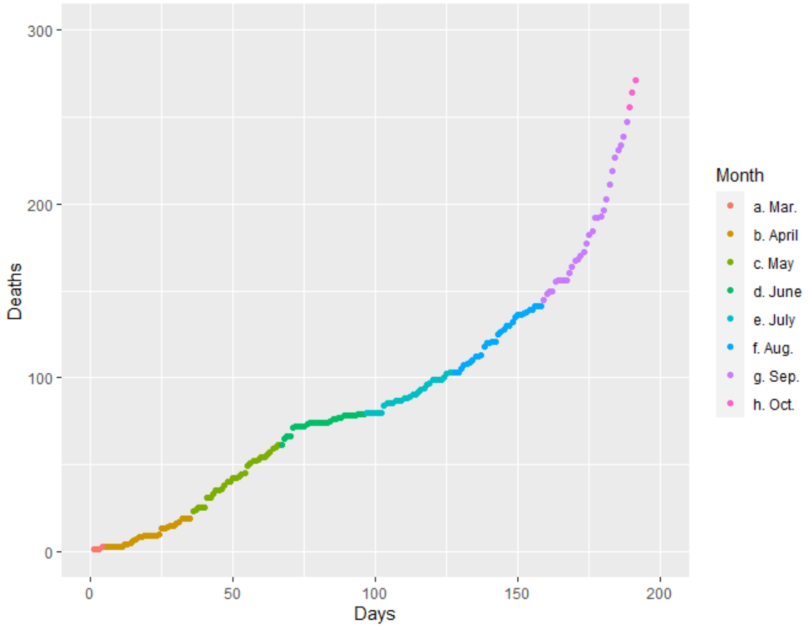
Fig. 1: Reported COVID-19 deaths in ND through Oct. 3rd
