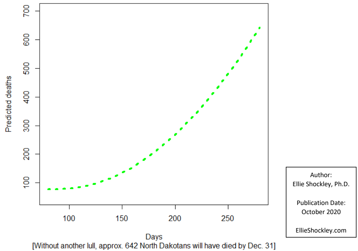
Fig. 3: Predicted COVID-19 deaths in ND through Dec. 31
