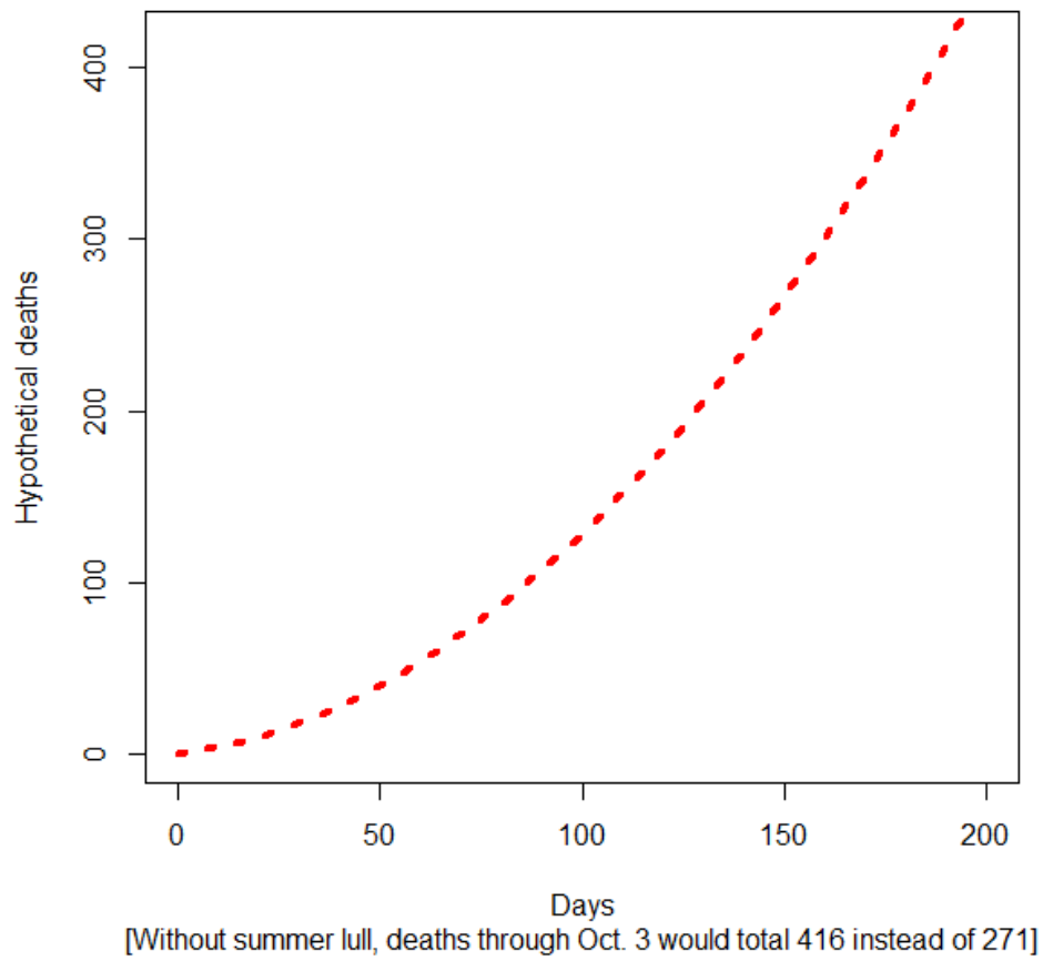
Fig. 2: Deaths through Oct. 3 if we lacked summer lull
